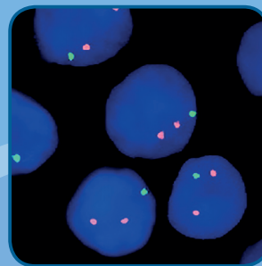
ATM/TP53
