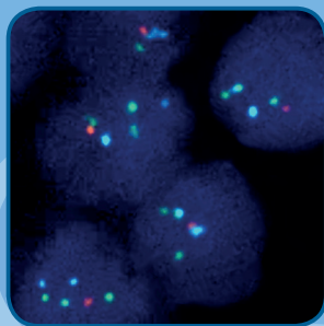
11q gain/loss
