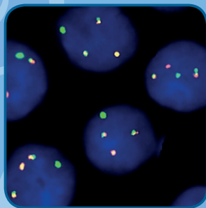
BCR/ABL1
